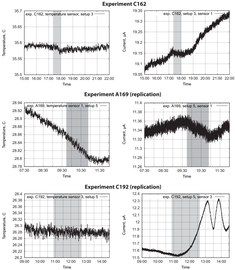
Figure 7. Impact of temperature variation on the sensors in laboratory B. Gray area represents the time when the container with irradiated water was placed close to the detector.
