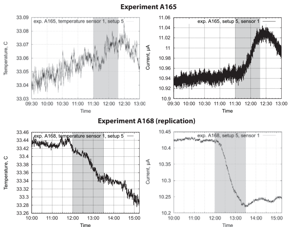
Figure 6. Impact of temperature variation on the sensors in laboratory B. Gray area represents the time when the LED generator was switched on. Variation of temperature 120 minutes before the experiment was about 0.02 C, and during the experiment 0.01 C.
